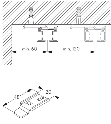
SG 3041 Bracket
